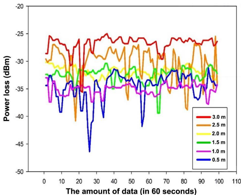
Figure 2. WiFi signal intensity for each receiver position.
