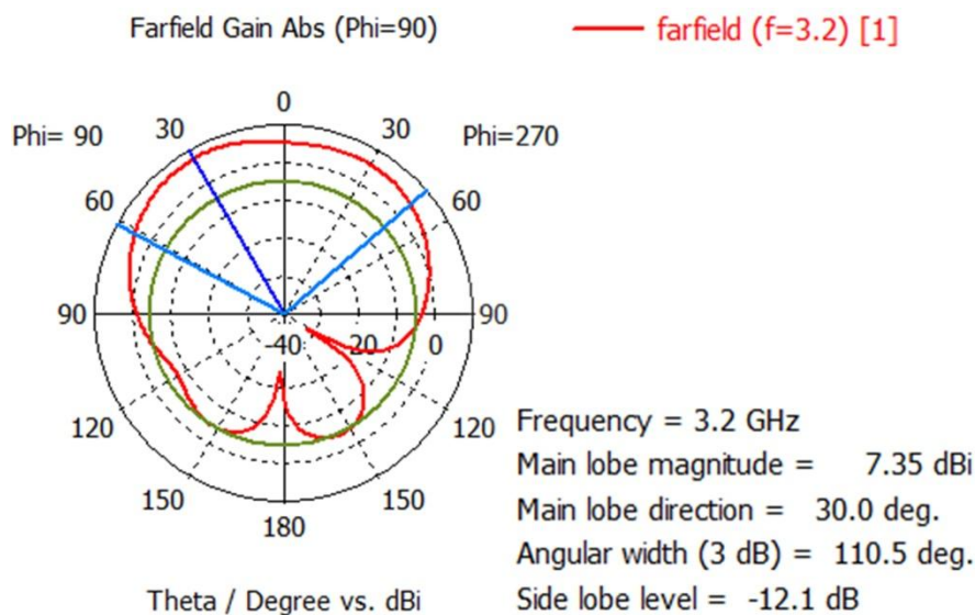
Figure 4. Farfield of antenna.
