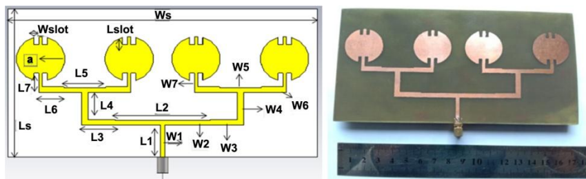
Figure 1. Microstrip antenna circular patch (front view).
