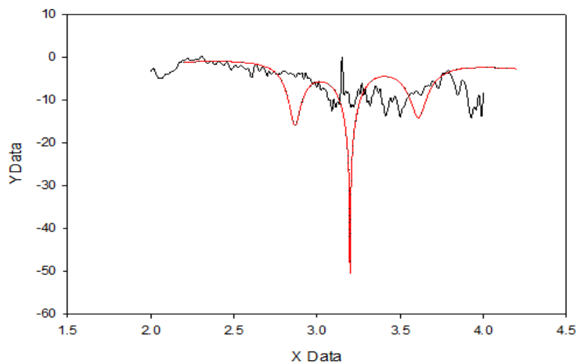
Figure 5. Measured vs simulated return loss.
