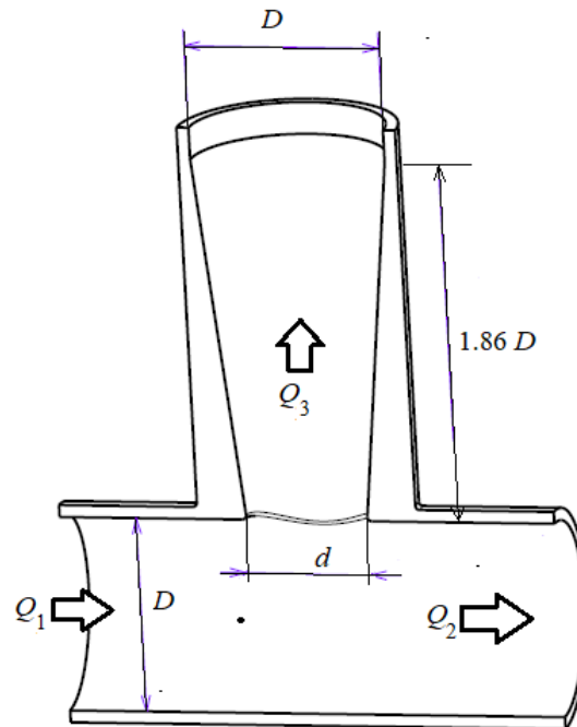
Figure 2. T-reduce junction
