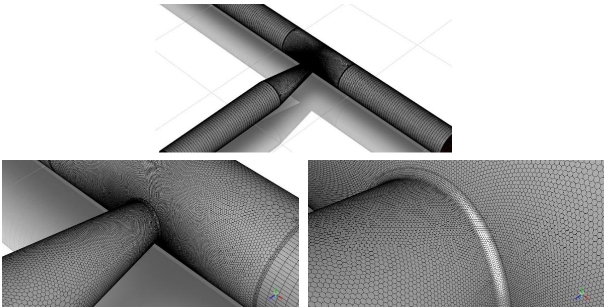
Figure 3. Meshing
