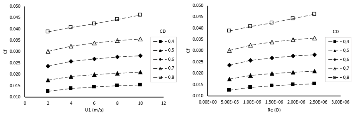
Figure 5. Flow coefficient against velocity and Re_D
