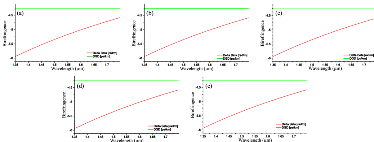
Figure 1. Birefringence results for (a) SMF-28, (b) SMF-28e, (c) SMF-28e+, (d) SMF-28e+LL, and (e) SMF-28ULL.
