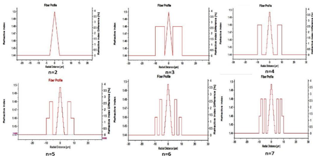
Figure 2. Refractive index profile of n layers
