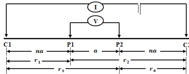
Figure 1. Schlumberger's rule [4]
