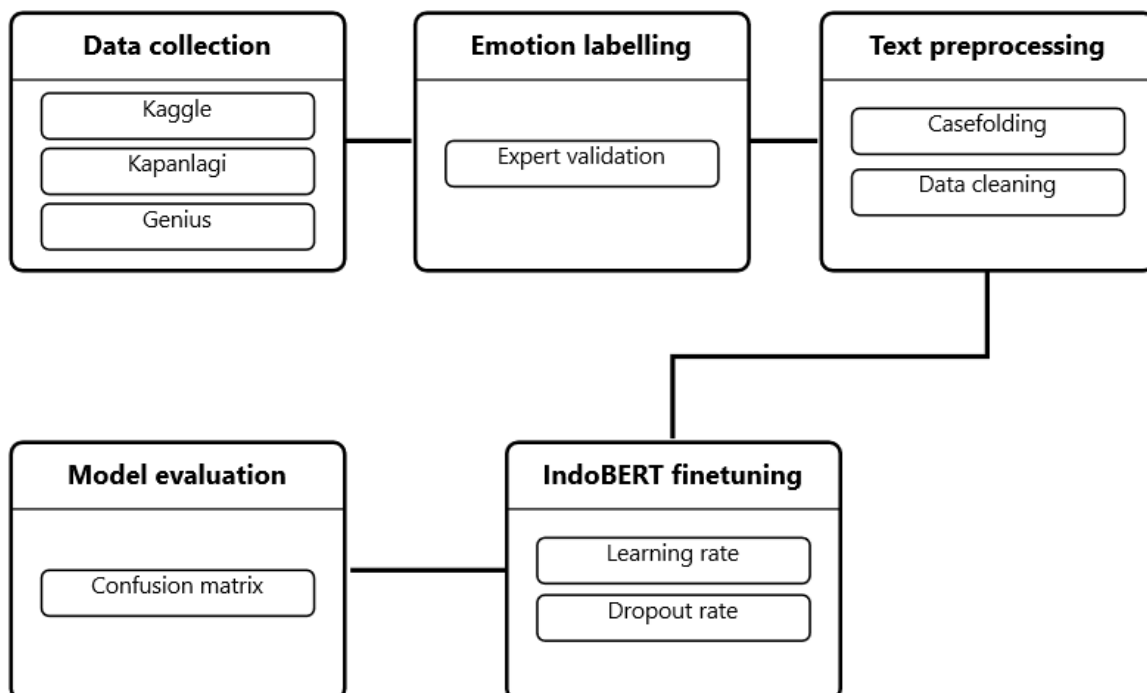
Figure 1. Research workflow.
