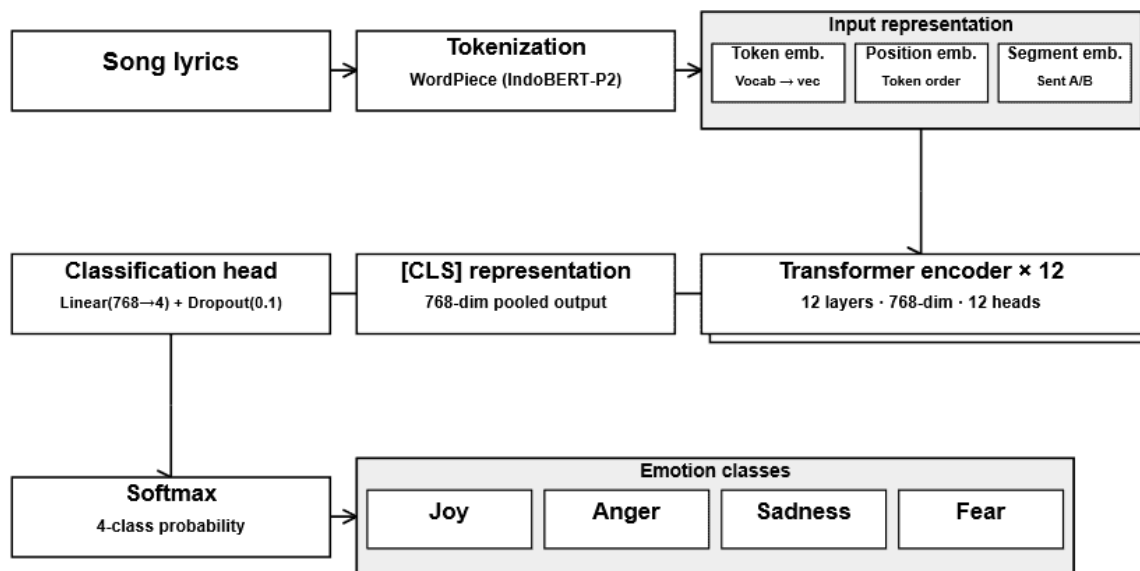
Figure 2. IndoBERT Architecture.
