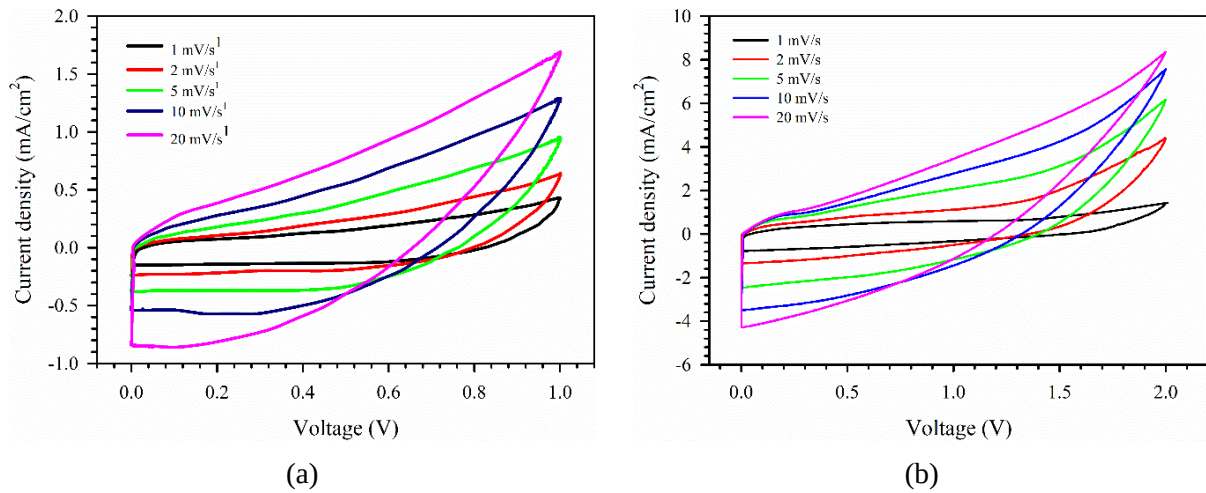
Figure 4. CV curves at voltage windows of (a) 1 V and (b) 2 V.
