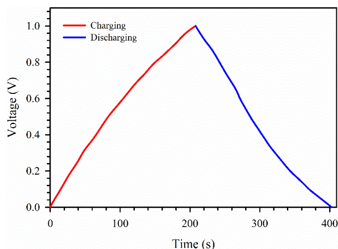
Figure 3. GCD curve at a voltage of 1 V.
