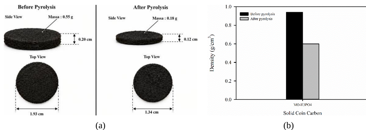
Figure 2. Physical changes in the pellet (a) and density comparison (b) before and after pyrolysis.
