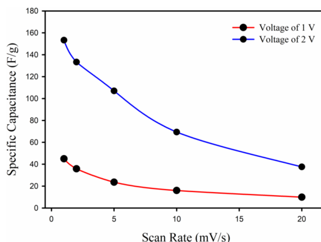
Figure 5. Specific capacitance as a function of scan rate at voltage windows of 0 – 1 V and 0 – 2 V.
