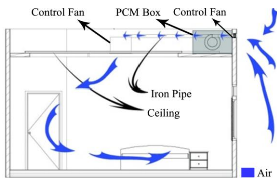
Figure 2. The working principle of EGACY.
